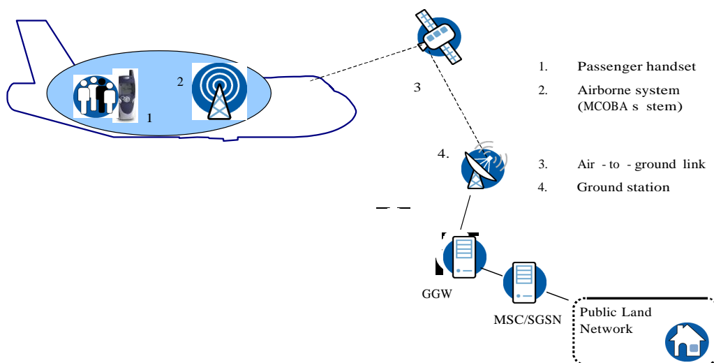
Figure C.1: Overview of the MCOBA system and associated transmission components
