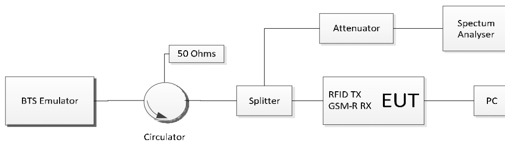
Figure 12: Set-up of equipment for mitigation test using splitter
