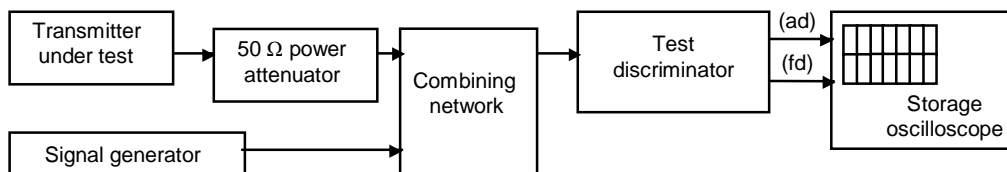
Figure 5: Measurement arrangement
