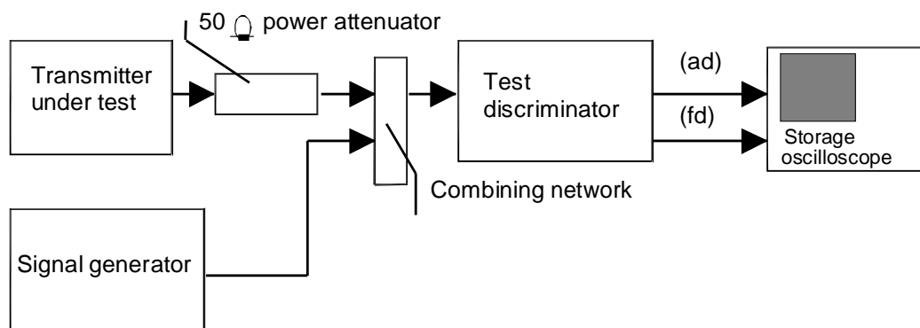
Figure 3: Measurement arrangement
